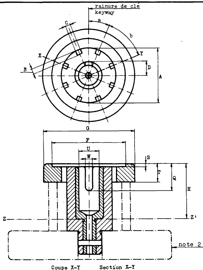
Coupe X-Y Section X-Y
