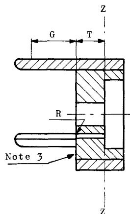
Coupe X-Y Section X-Y
